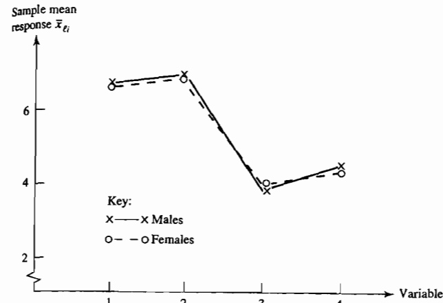
Figure 6.5 Sample profiles for marriage-love responses.
