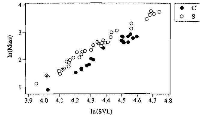
Figure 6.7 Scatter plot of \ln(\text{Mass}) versus \ln(\text{SVL}) for the lizard data in Table 6.7.
