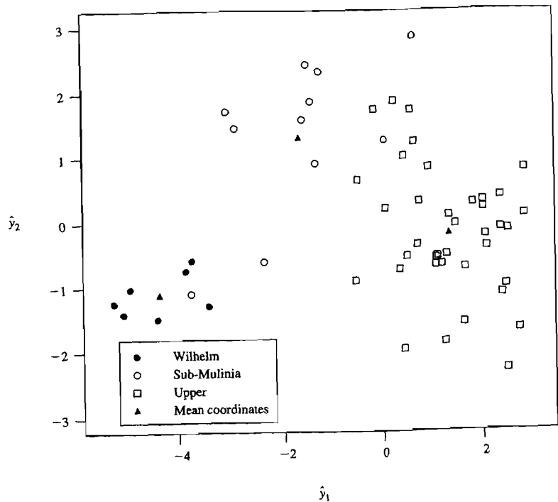
Figure 11.12 Crude-oil samples in discriminant space.
