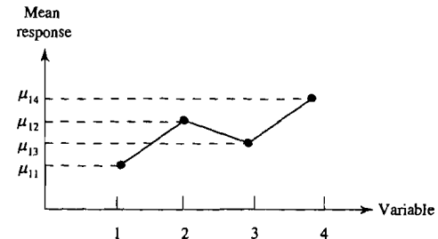
Figure 6.4 The population profile p = 4 .
