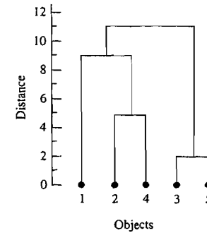
Figure 12.6 Complete linkage dendrogram for distances between five objects.
