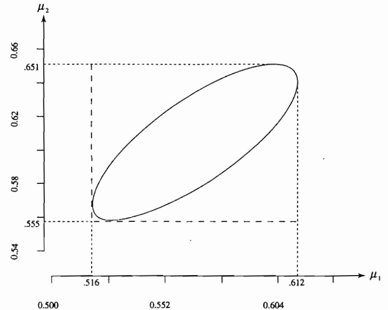
Figure 5.2 Simultaneous T^2 -intervals for the component means as shadows of the confidence ellipse on the axes—microwave radiation data.
