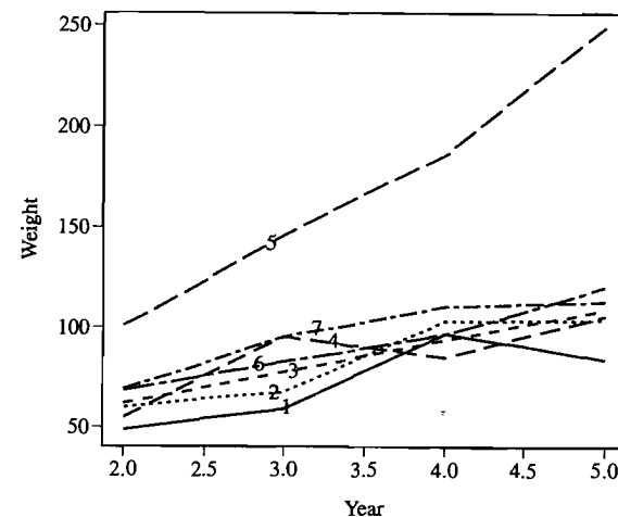
Figure 1.13 Combined growth curves for weight for seven female grizzly bears.
