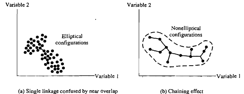
Figure 12.5 Single linkage clusters.
