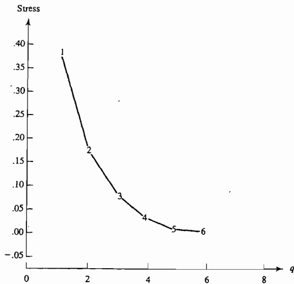
Figure 12.17 Stress function for distances between utilities.
