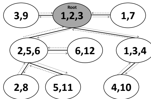
Figure 2: One possible clique tree for the genotype network above.
