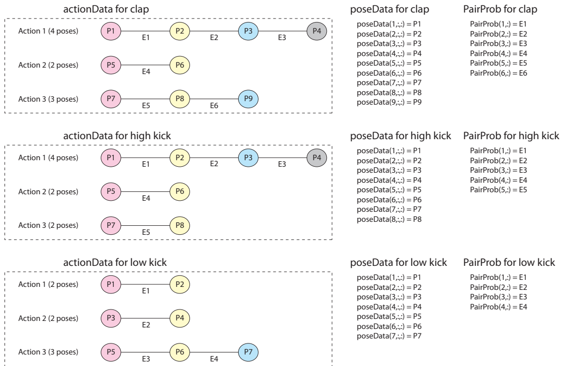
Figure 3: Illustration of the data structures used for this part. Note that each actionData / poseData / PairProb structure will only contain data for a single action class. The actionData structure uses margin to index where to find the poses in poseData and pair to index where to find the edges in PairProb . For example, the first pose in Action 2 of the “clap” action can be found in the 5th row of poseData , and the edge between the first and second poses of Action 2 can be found in the 4th row of PairProb .
