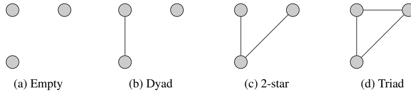
Figure 8: Triads
