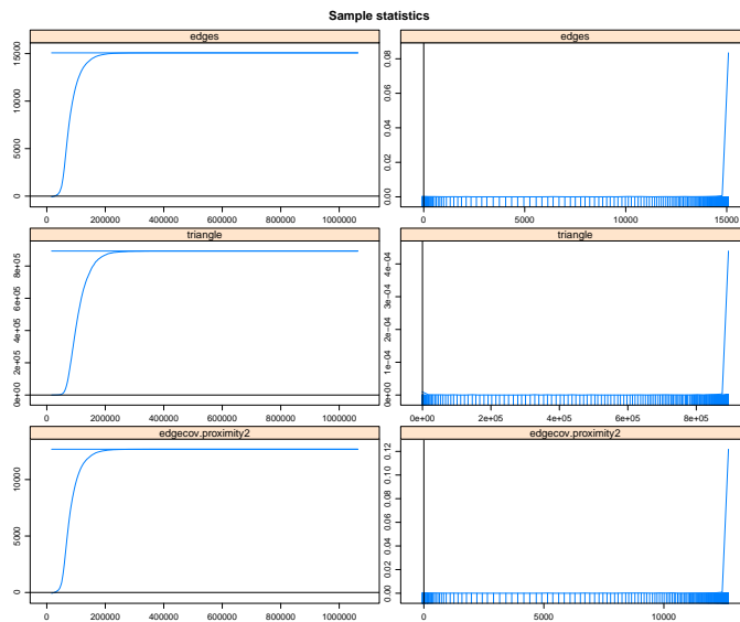
Figure 15: Goodness of Fit diagnostics, bad example
