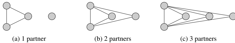
Figure 10: Shared partners
