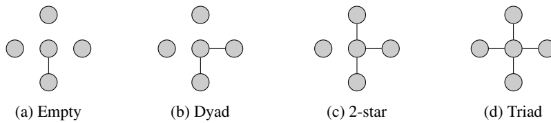
Figure 9: K-stars
