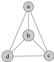
Figure 4: Markov graph
