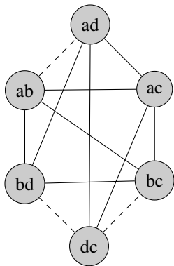
Figure 6: Dependence graph and configuration identification
