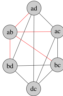
Figure 5: Dependence graph
