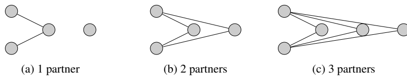
Figure 11: Shared partners (dyadic)
