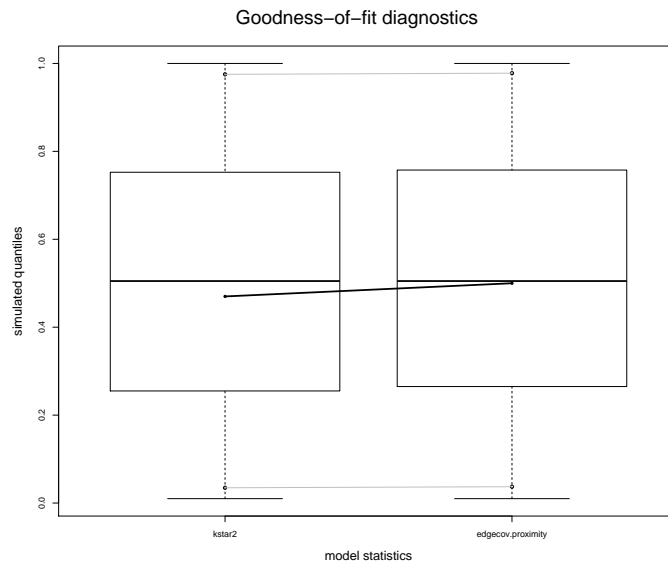
Figure 16: GOF: boxplot analysis
