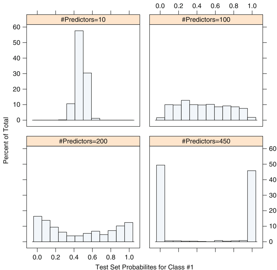
Fig. 12.11: Histograms of test set class probabilities for a simulated two-class example where all predictors are non-informative. As the number of predictors approaches the number of samples (500 in the training set), the class probabilities begin to diverge towards the two extremes (however, the overall accuracy remains near 50 %)
