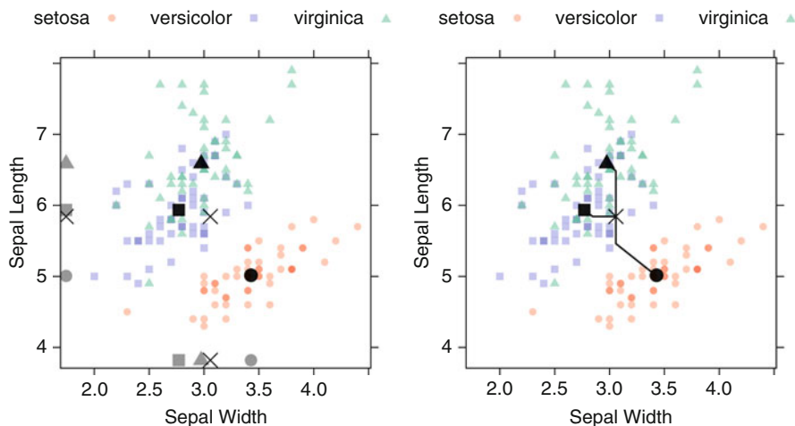
Fig. 12.18: Left : An example with three classes, their class-specific centroids (in black), and the overall centroid (×). The grey symbols along the axes are the centroids projected down into a single dimension. Right : The paths of the class centroids when shrunken to the center of the distributions
