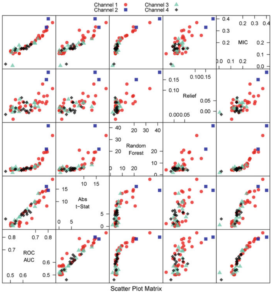
Fig. 18.6: A scatter plot matrix of several different metrics for ranking predictors with the image segmentation data set
